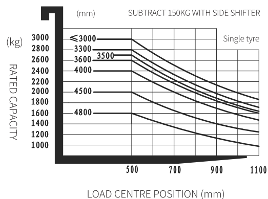
EFX302 RATED CAPACITIES AND LOAD CENTERS GRAPH
